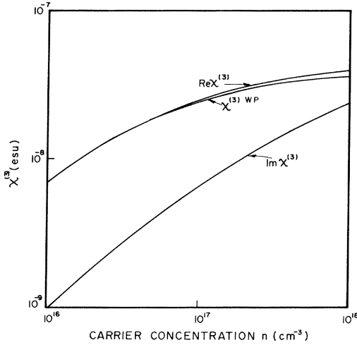
FIG. 2. Variation of real and imaginary parts of \chi_{xxxx}^{(3)}(\omega_a, \omega_a, -\omega_b) \equiv \chi^{(3)} with the carrier concentration n for degenerate InSb. \chi^{(3)WP} denotes the values obtained by neglecting collisions.
